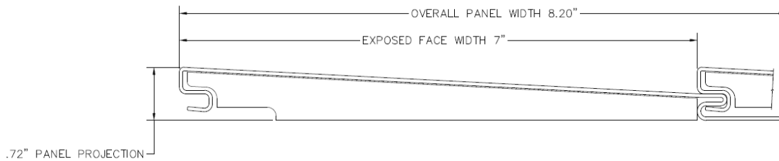
FIGURE 1 – ASCEND™ Composite Cladding Profile
